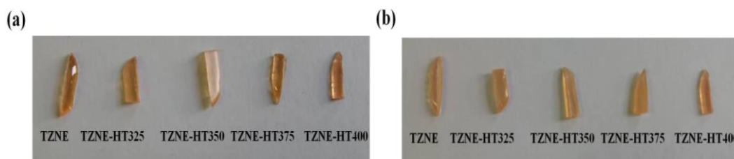
Fig. 2. Physical appearance of tellurite glass (a) before immersion in distilled water (b) after 10 days of immersion in distilled water.
